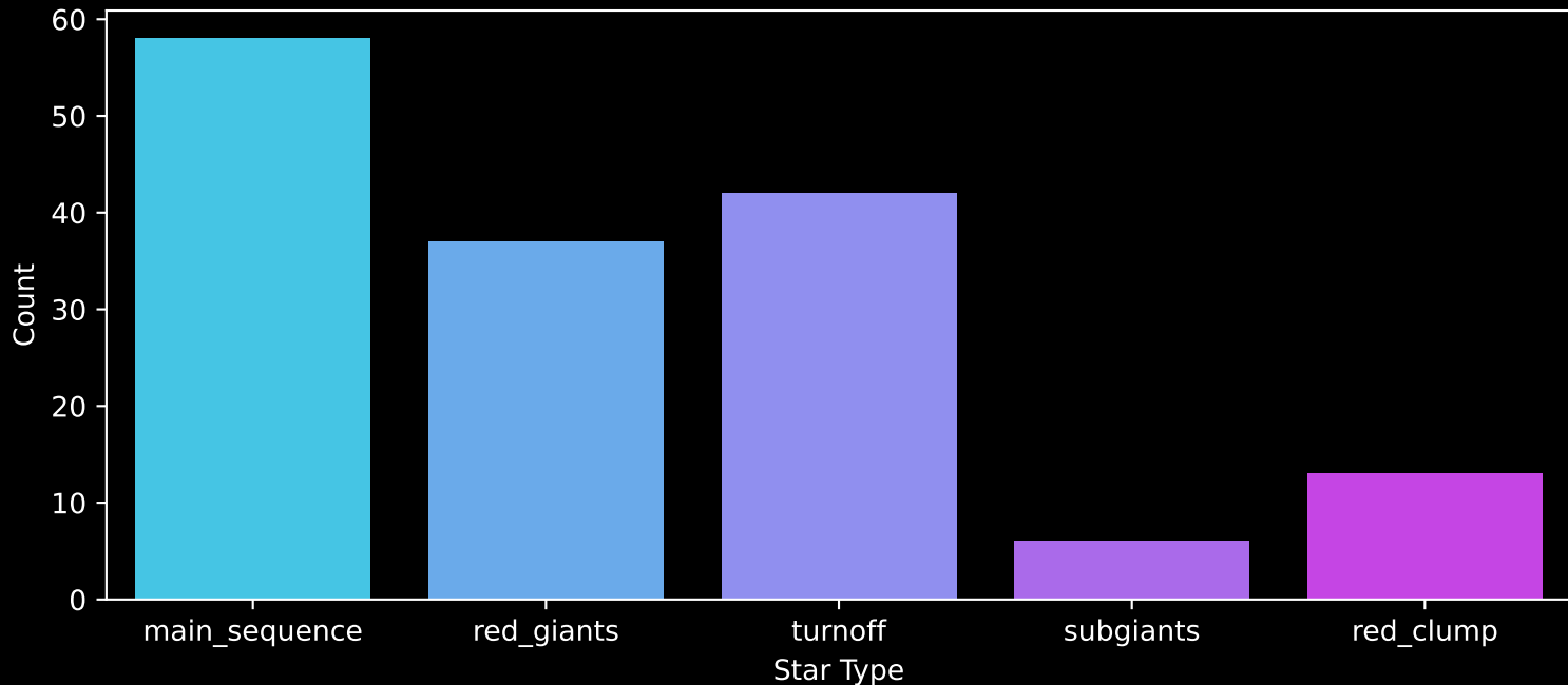
APOGEE DR17 Field: [calibration] Count plot of Star Type
