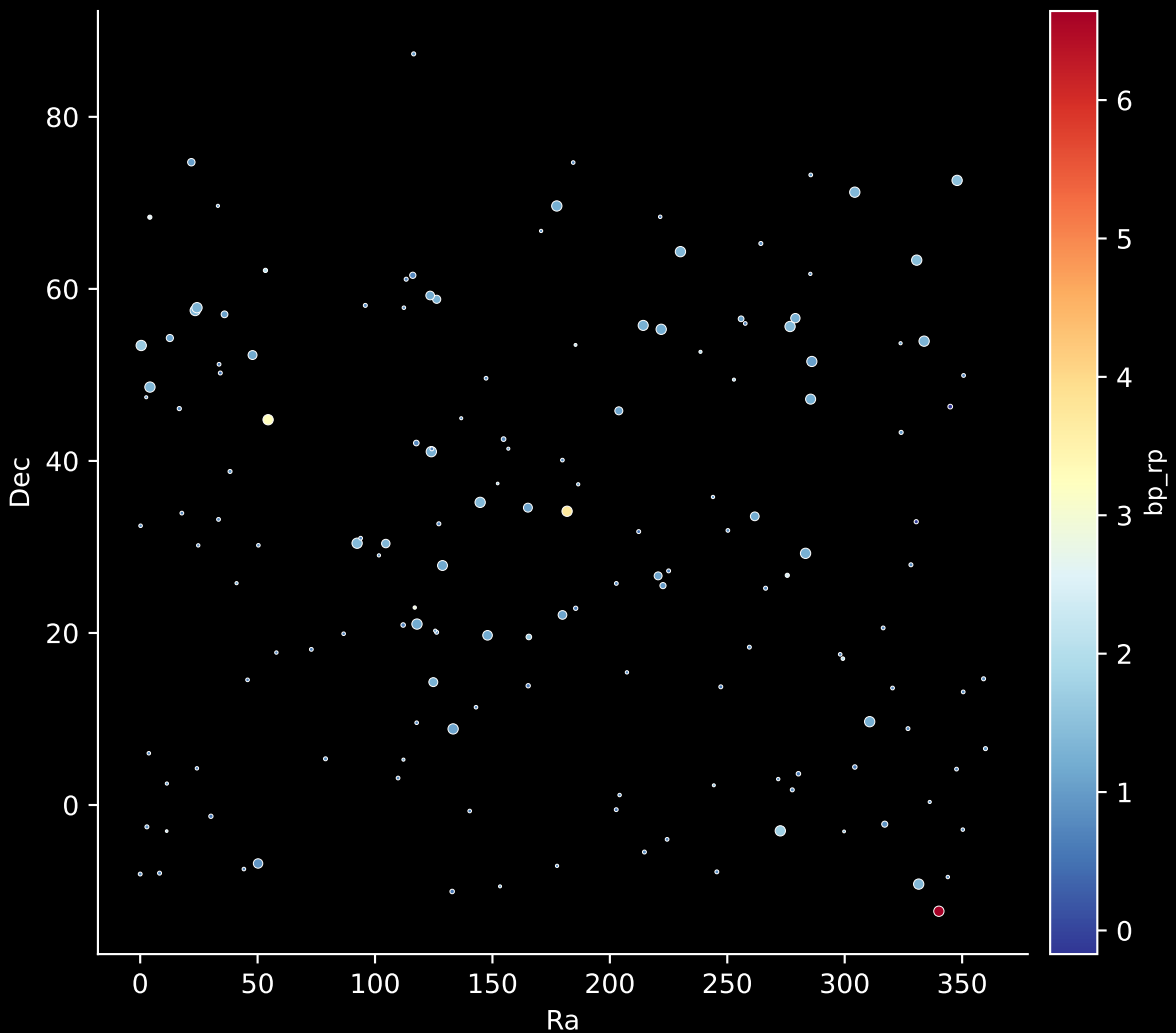
APOGEE DR17 Field: [calibration] Stars: 156
