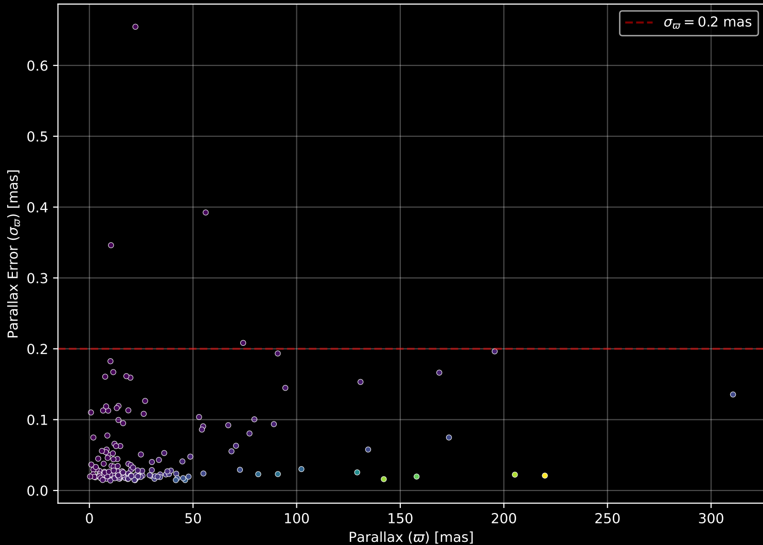
APOGEE DR17 Field: [calibration] Parallax Quality (n= 156)
