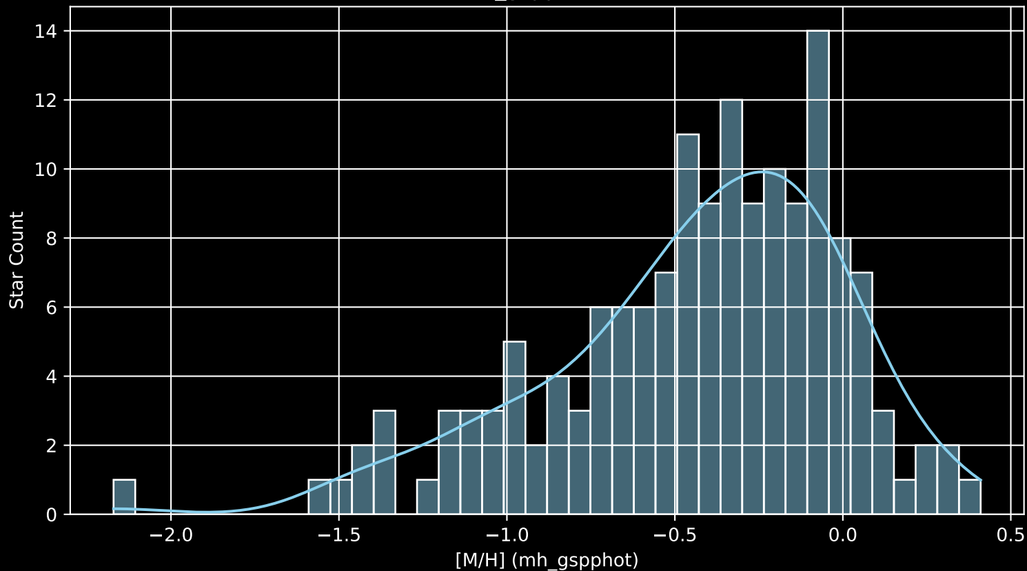
APOGEE DR17 Field: [calibration [M/H] (mh_gspphot) (n= 155)
