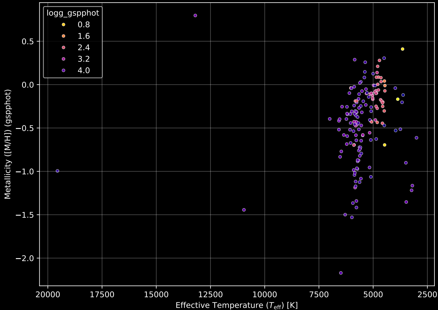
APOGEE DR17 Field: [calibration] Stellar Population Parameters (n= 156)
