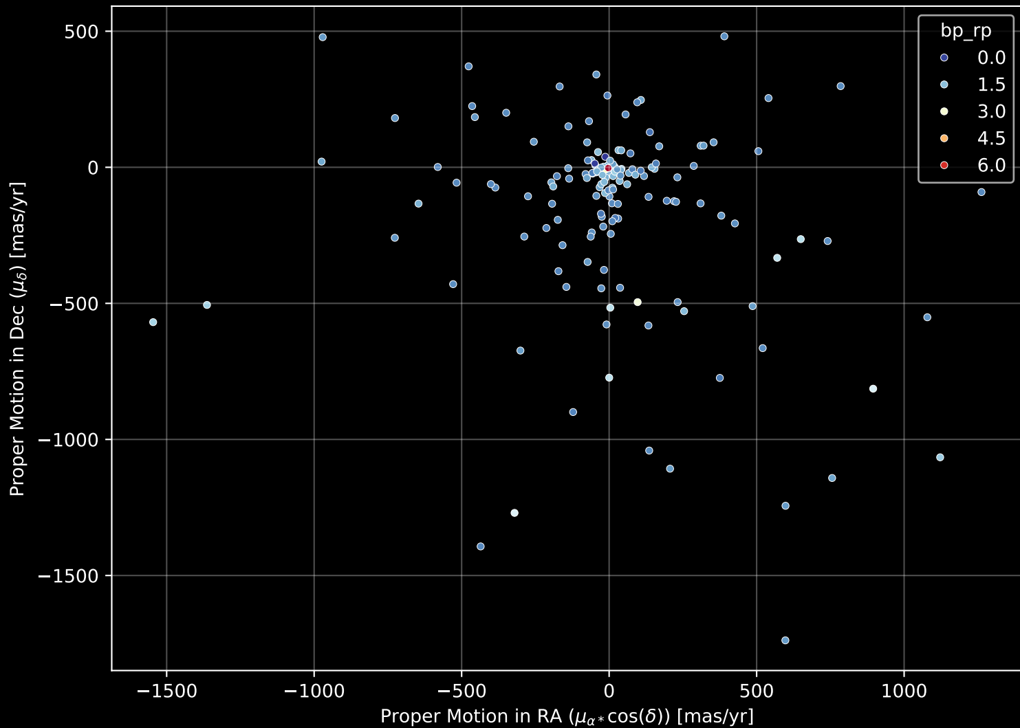
APOGEE DR17 Field: [calibration] Proper Motion Diagram (n= 156)
