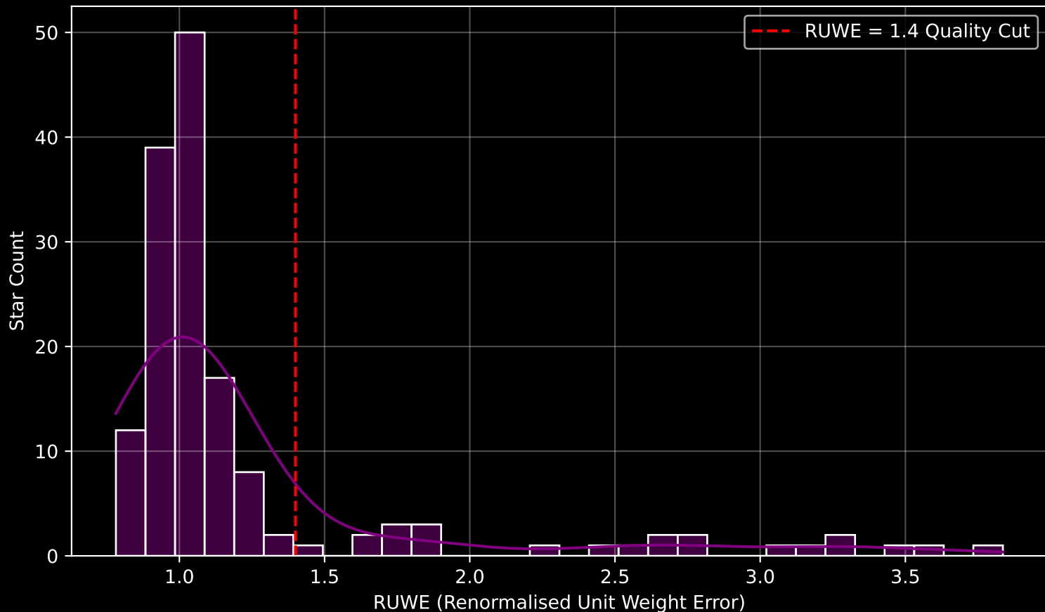
GAPOGEE DR17 Field [calibration] RUWE Distribution (n= 151)
